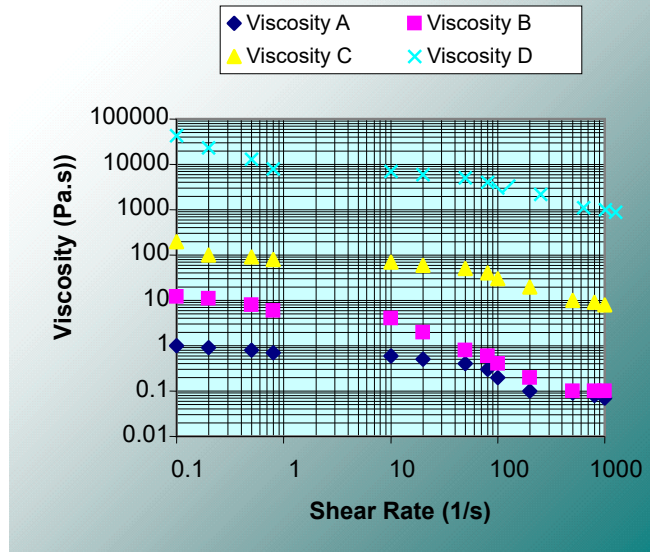
Figure 3: Non-Newtonian Fluids
